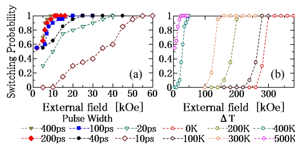
Fig.3. Magnetization reversal probability for various thermal pulse width T_w (a), and magnitude \Delta T (b).
